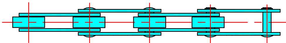
HOLLOW PINS
